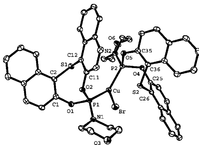
Figure 3. Molecular structure of 8a . Solvent molecules and all hydrogen atoms have been omitted for clarity. Displacement ellipsoids are drawn at the 50% probability level.
