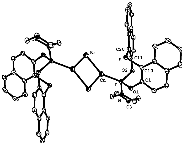
Figure 1. Molecular structure of 5a . All hydrogen atoms have been omitted for clarity. Displacement ellipsoids are drawn at the 50% probability level.
