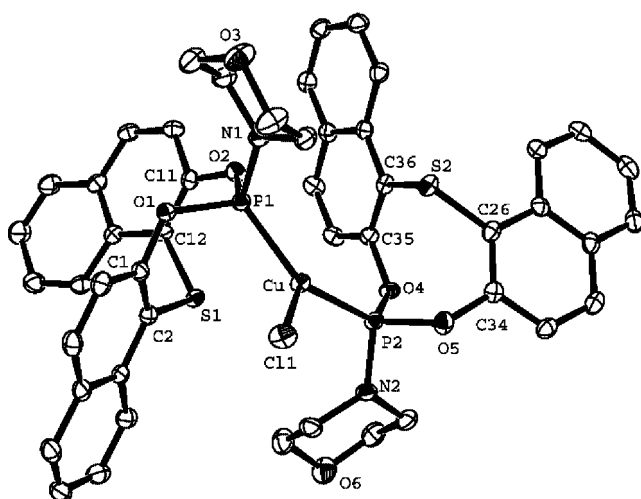
Figure 2. Molecular structure of 7a ·CH 2 Cl 2 . Solvent molecules and all hydrogen atoms have been omitted for clarity. Displacement ellipsoids are drawn at the 50% probability level.
