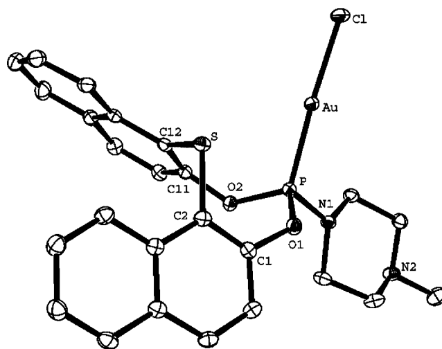
Figure 5. Molecular structure of 13b . All hydrogen atoms have been omitted for clarity. Displacement ellipsoids are drawn at the 50% probability level.
