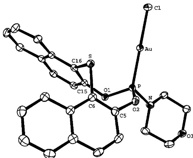
Figure 4. Molecular structure of 13a . All hydrogen atoms have been omitted for clarity. Displacement ellipsoids are drawn at the 50% probability level.
