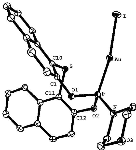
Figure 6. Molecular structure of 14a . All hydrogen atoms have been omitted for clarity. Displacement ellipsoids are drawn at the 50% probability level.
